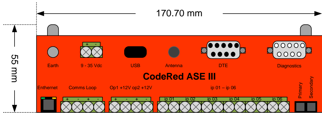
ASE III Main Unit - Back View
