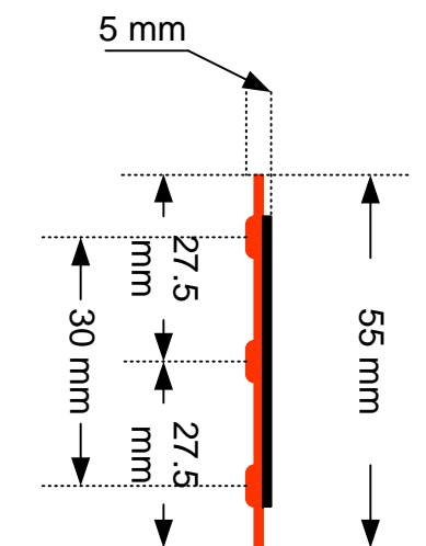
ASE III Fixing Bracket with 3M Industrial Velcro Side View
