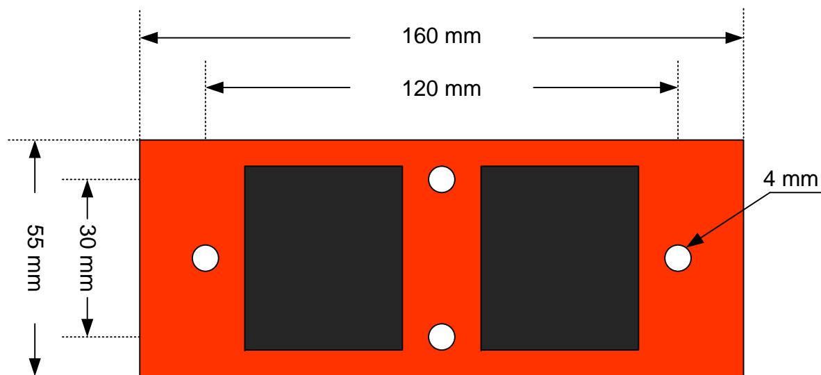
ASE III Fixing Bracket with 3M Industrial Velcro
